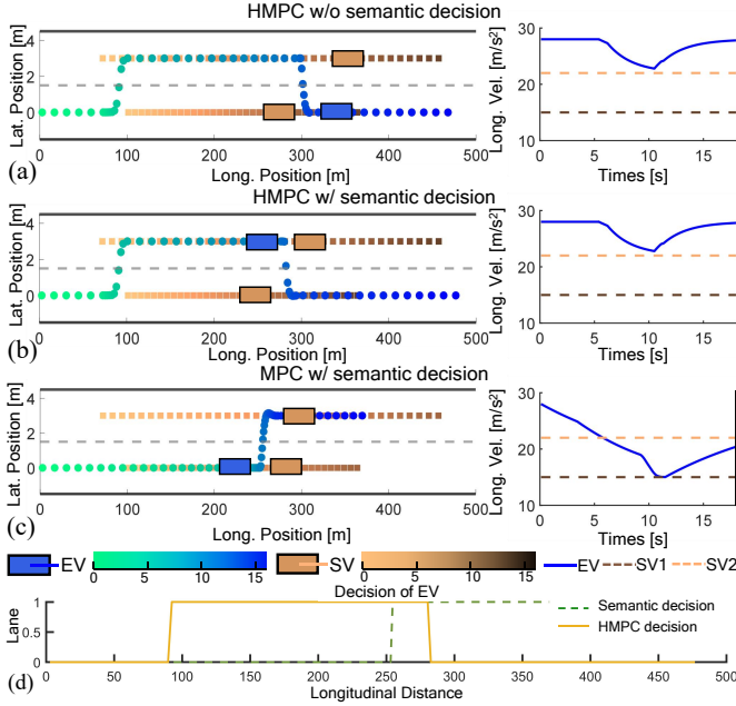
Fig. 9. Results of simulation experiment case 2. (a)-(c) Vehicle trajectory during an overtaking maneuver with key moments indicated and corresponding longitudinal speed profile. (d) Comparison between the semantic decision and the HMPC decision (with the semantic decision).
