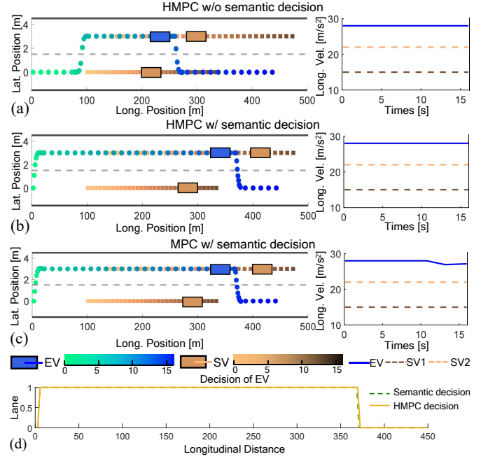
Fig. 8. Results of simulation experiment case 1. (a)-(c) Vehicle trajectory during an overtaking maneuver with key moments indicated and corresponding longitudinal speed profile. (d) Comparison between the semantic decision and the HMPC decision (with the semantic decision).
