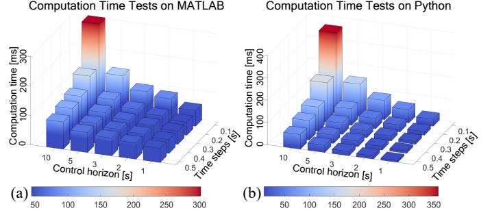
Fig. 12. Computation time of various control horizons and time steps. The tests in nuPlan and the real-world are both based on Python.
