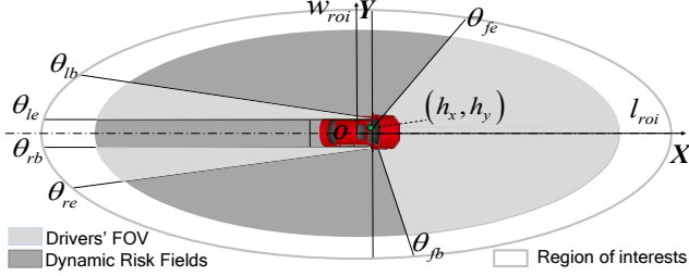
Fig. 3. Asymmetric risk field based on the driver's FOV. X and Y represent the coordinate axes of the SV's coordinate system, l_{roi} and w_{roi} indicating the driver's region of interests (ROI) in the longitudinal and lateral directions, which are set manually.
