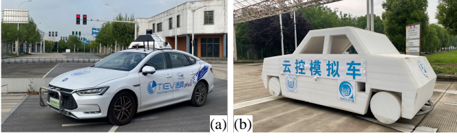
Fig. 13. (a) Experiment vehicle. (b) Cloud-controlled simulated vehicle.
