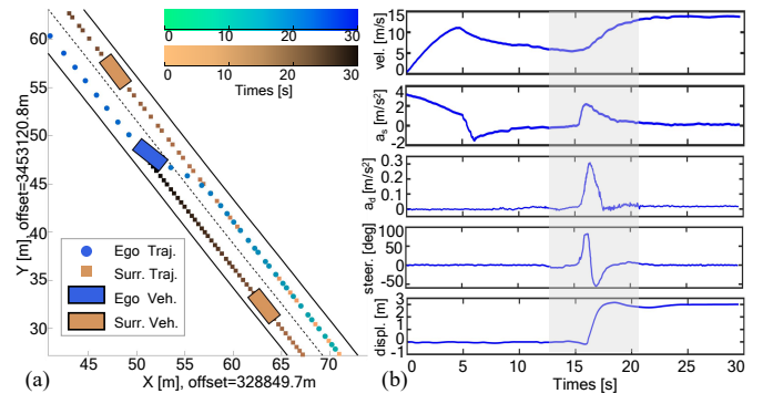
Fig. 15. (a) Vehicle trajectory visualization. (b) Results of real-world test, shown from top to bottom, illustrate the EV's velocity, longitudinal acceleration a_s , lateral acceleration a_d , steering wheel angle, and lateral displacement during the overtaking process over time.
