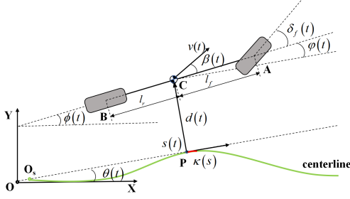
Fig. 5. Kinematic vehicle model in the Frenét coordinate system.
