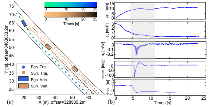
Fig. 16. (a) Vehicle trajectory visualization. (b) Results of real-world test, shown from top to bottom, illustrate the EV's velocity, longitudinal acceleration a_s , lateral acceleration a_d , steering wheel angle, and lateral displacement during the overtaking process over time.
